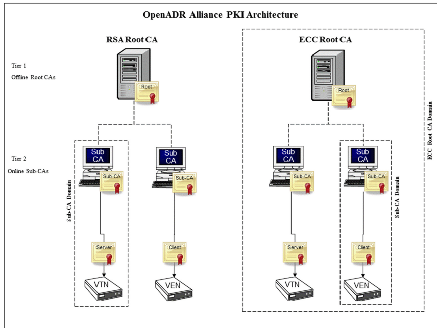
Figure 2 OpenADR PKI Architecture
