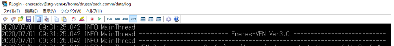
Photo 1: FW Version
